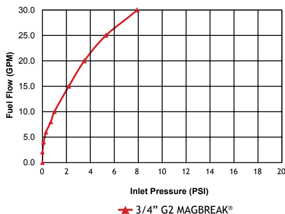
008330 3/4" G2 MagBreak® Reconnectable STB Back Pressure Performance
