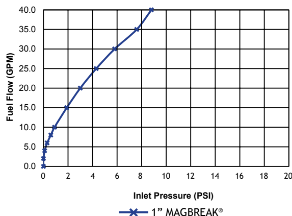
008331 1" MagBreak® Reconnectable STB Back Pressure Performance
