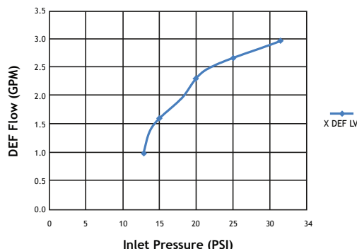
X DEF LV Nozzle Back Pressure Performance
