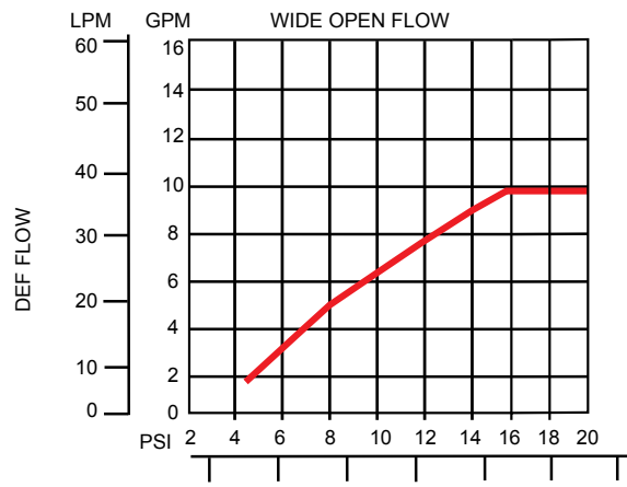
SST DEF NOZZLE AVERAGE BACK PRESSURE PERFORMANCE VERIFICATION
